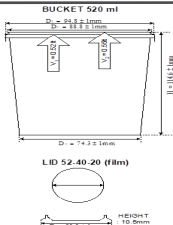
PRODUCT DRAWING & LIDS
